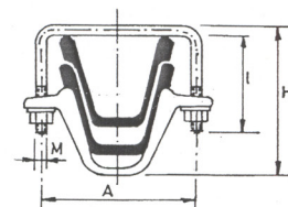
UNION GRAPA ABARCON PERFIL "TH"
