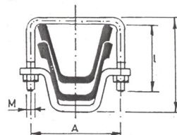
UNION GRAPA ADAPTADA ABARCON PERFIL "TH"
