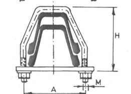
UNION LLANTA ABARCON PERFIL "TH-INV"
