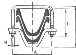
UNION GRAPA ADAPTADA ABARCON PERFIL "THN"
